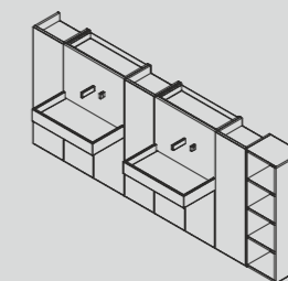
CONJUNTO 240 Assembly | Ensemble
